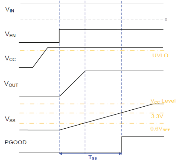
Figure 3. Soft-start Sequence of AOZ22559QI
