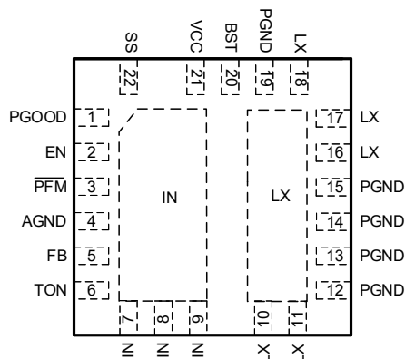
AOZ2261BQI-20 22-pin 4mm x 4mm QFN
