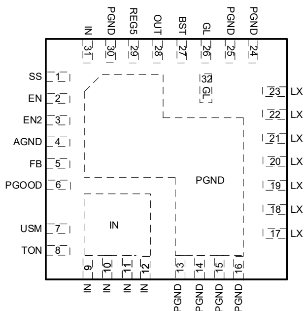
AOZ2295QI-05 31-Pin 4mm x 4mm QFN
