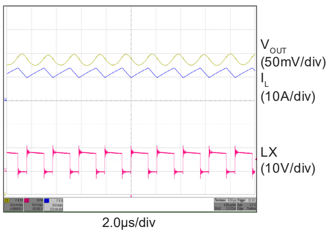
Normal Operation ( V_{IN} = 8\text{V} , I_{OUT} = 12\text{A} )
