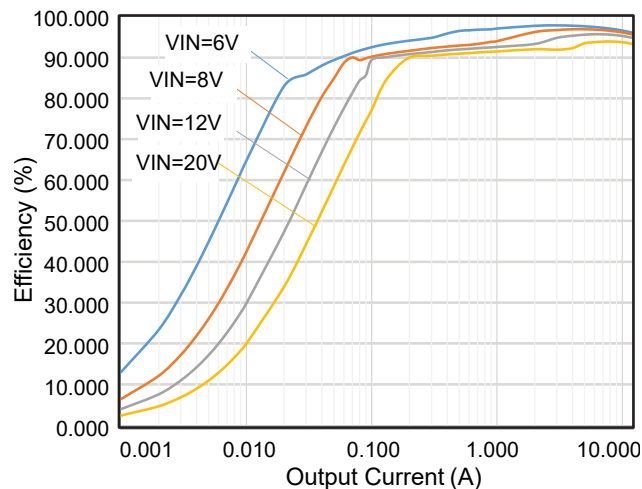
Figure 2. Efficiency (USM) V_{OUT} = 6\text{V}/8\text{V}/12\text{V}/20\text{V} , I_{OUT} = 1\text{mA} \sim 12\text{A}
