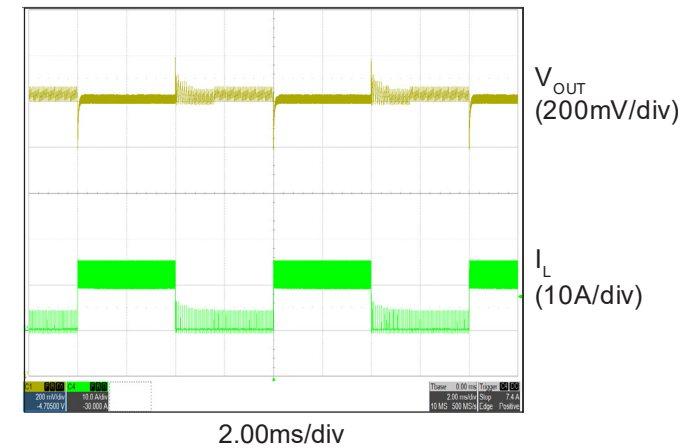
Load Transient ( V_{IN} = 6\text{V} , I_{OUT} = 0\text{A} \sim 12\text{A} @ \text{SR} = 2.5\text{A}/\mu\text{s} )
