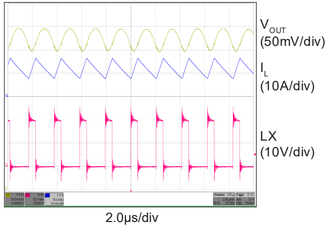
Normal Operation ( V_{IN} = 12\text{V} , I_{OUT} = 12\text{A} )
