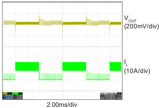
Load Transient ( V_{IN} = 8\text{V} , I_{OUT} = 0\text{A} \sim 12\text{A} @ \text{SR} = 2.5\text{A}/\mu\text{s} )
