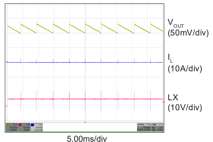
Normal Operation ( V_{IN} = 8\text{V} , I_{OUT} = 0\text{A} )
