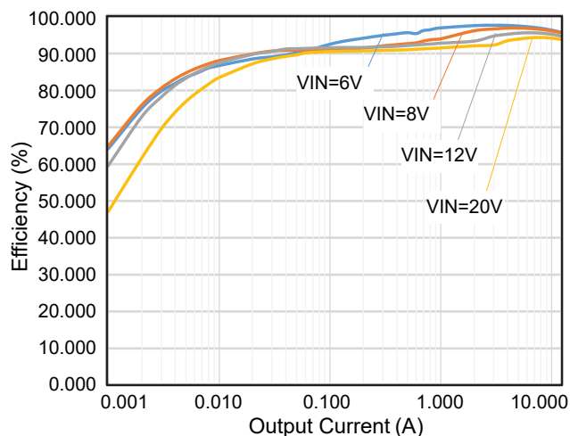
Figure 1. Efficiency V_{OUT} = 6\text{V}/8\text{V}/12\text{V}/20\text{V} , I_{OUT} = 1\text{mA} \sim 12\text{A}
