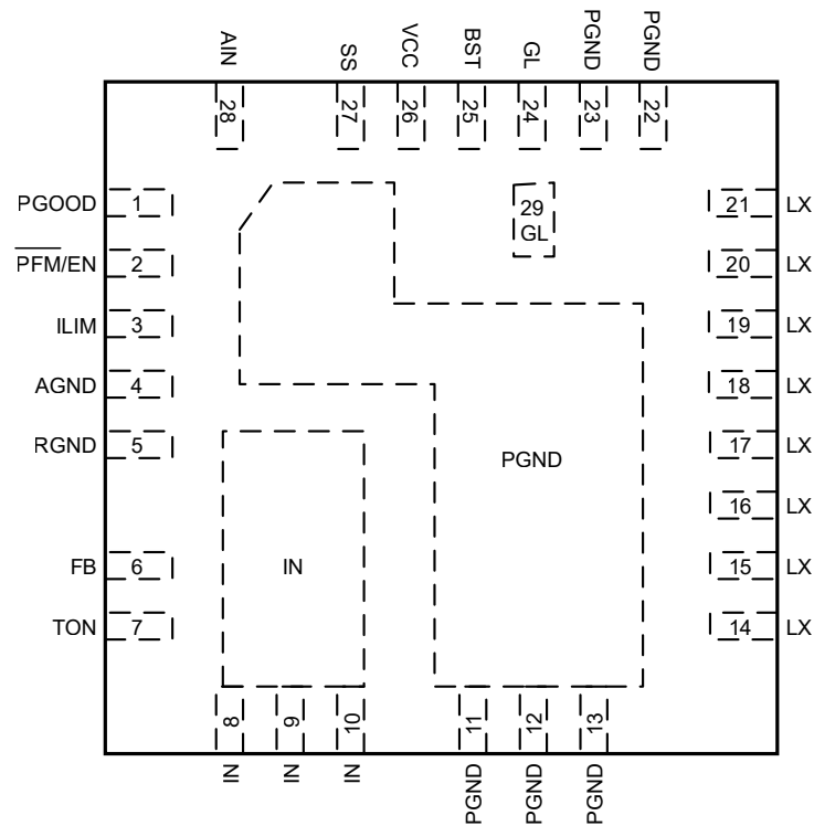
AOZ2387QI 28-pin 5mm x 5mm QFN
