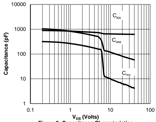
Figure 8: Capacitance Characteristics
